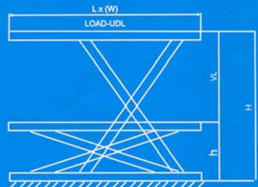
UDL - Uniformly Distributed Load
